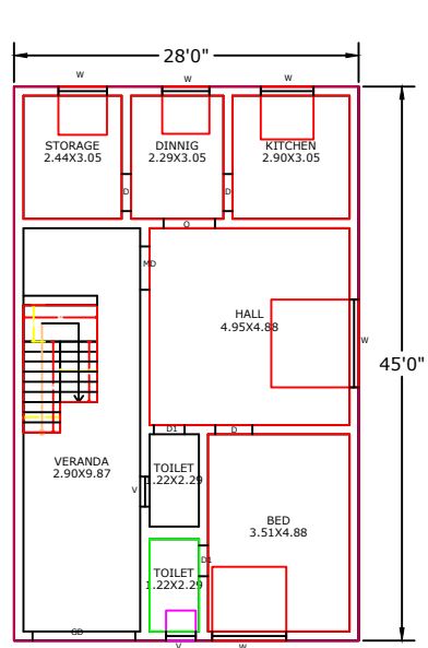
EXG.GROUND FLOOR PLAN
