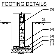
SECTION
