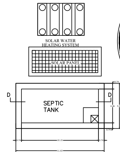
PLAN OF SEPTIC TANK SCALE 1"=2'0"
