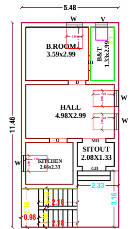
PRO.GROUND FLOOR PLAN
