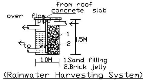
(Rainwater Harvesting System)
