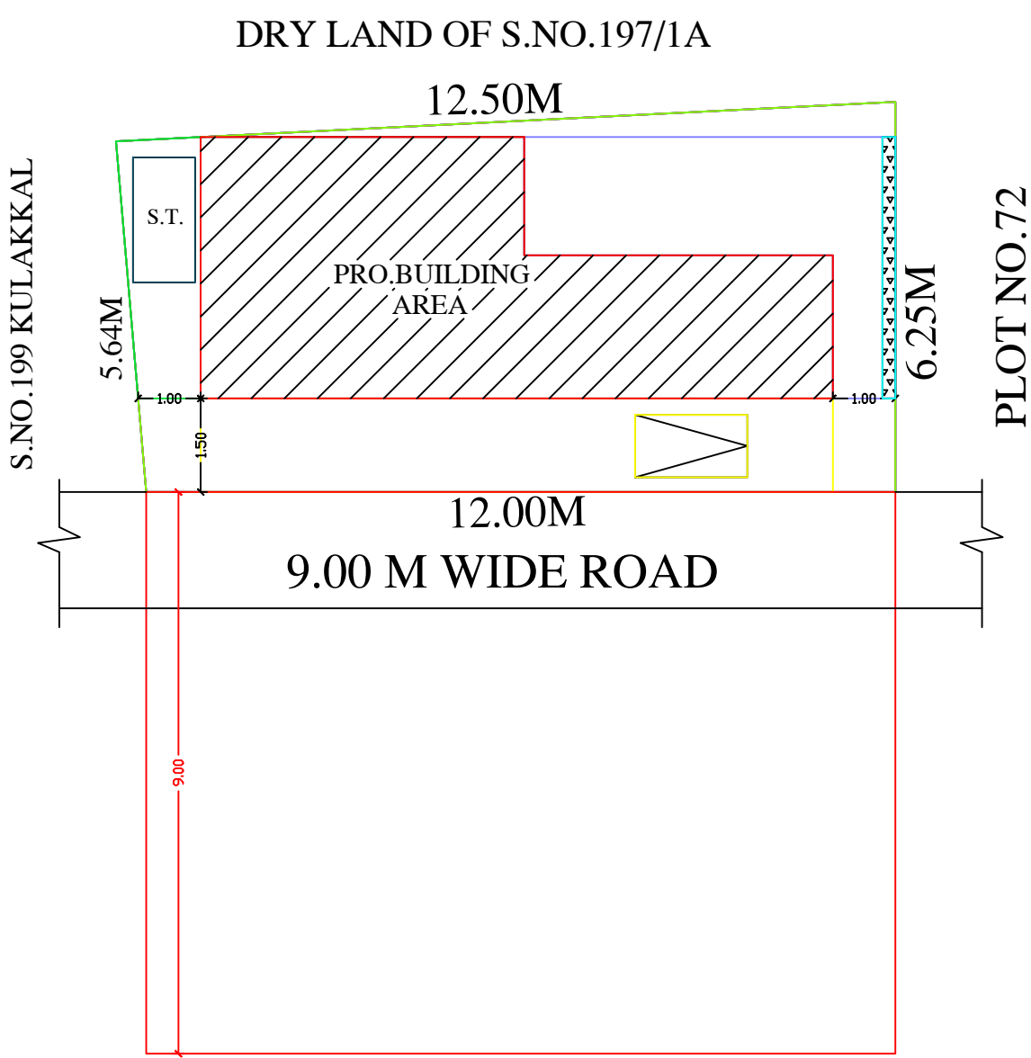
SITE PLAN
