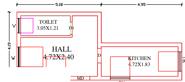
ND FLOOR PLAN
