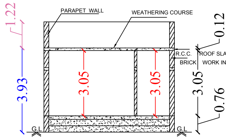
Section on-"AA"
