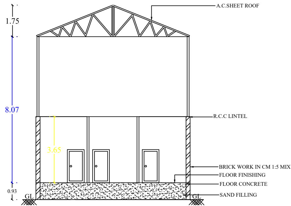
SECTION A1-A1
