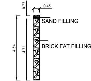
DETAILS OF PERCULATION PIT
