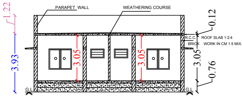
Section on-"AA"
