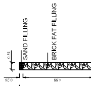
DETAILS OF PERCUSSION PIT
