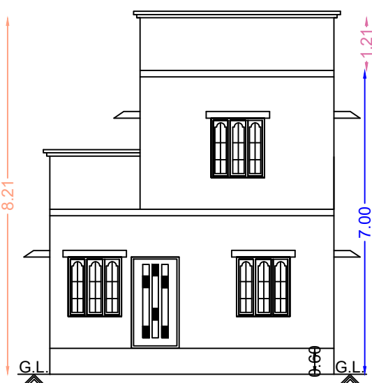
Front Elevation
