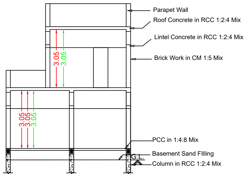
Section RR
