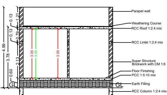
SECTION ON "VR"
