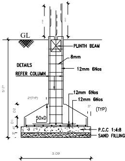
FOUNDATION DETAILS
