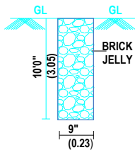
PERCULATION PIT
