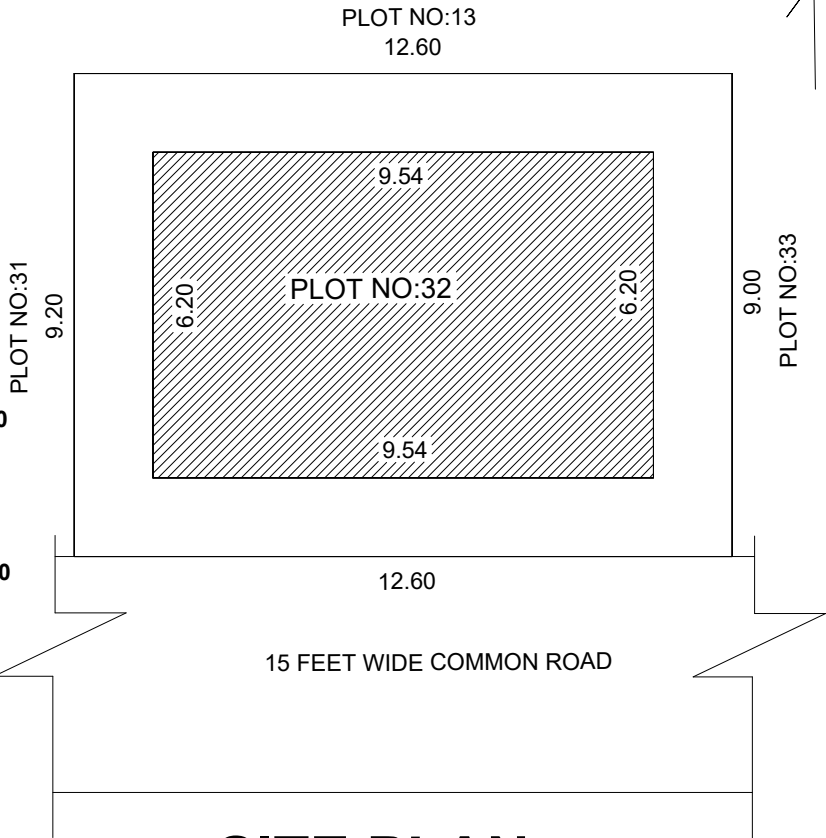
SITE PLAN
