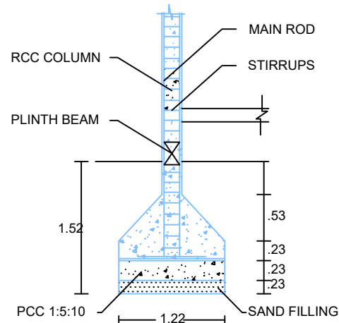
COLUMN DETAILS
