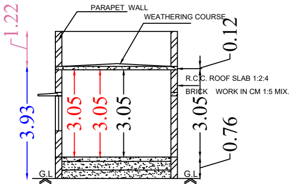
Section on-"AA"
