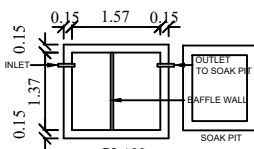
SEPTIC TANK
