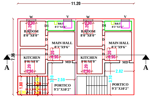
PRO.GROUND FLOOR PLAN
