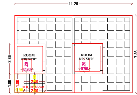
PRO.FIRST FLOOR PLAN
