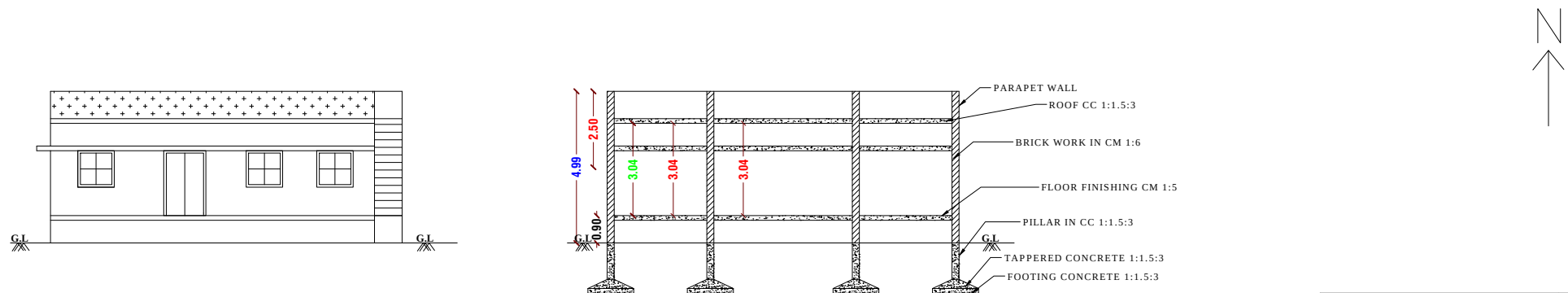
FRONT ELEVATION
