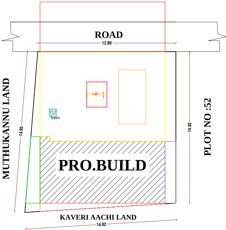
SITE PLAN
