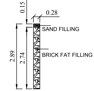
DETAILS OF PERCULATION PIT
