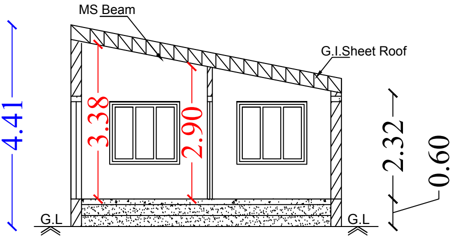
Section on-"AA"
