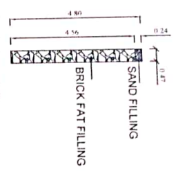
DETAILS OF PERCUSSION PIT
