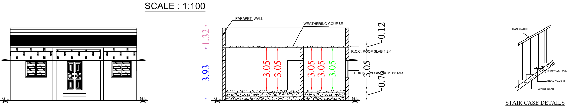
STAIR CASE DETAILS
