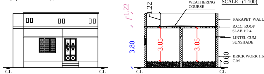
FRONT ELEVATION
