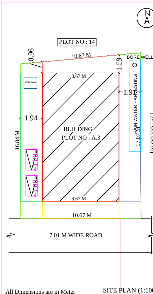
SITE PLAN (1:100)
