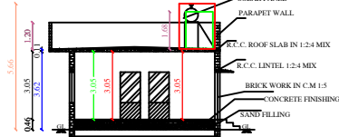
SECTION ON AA
