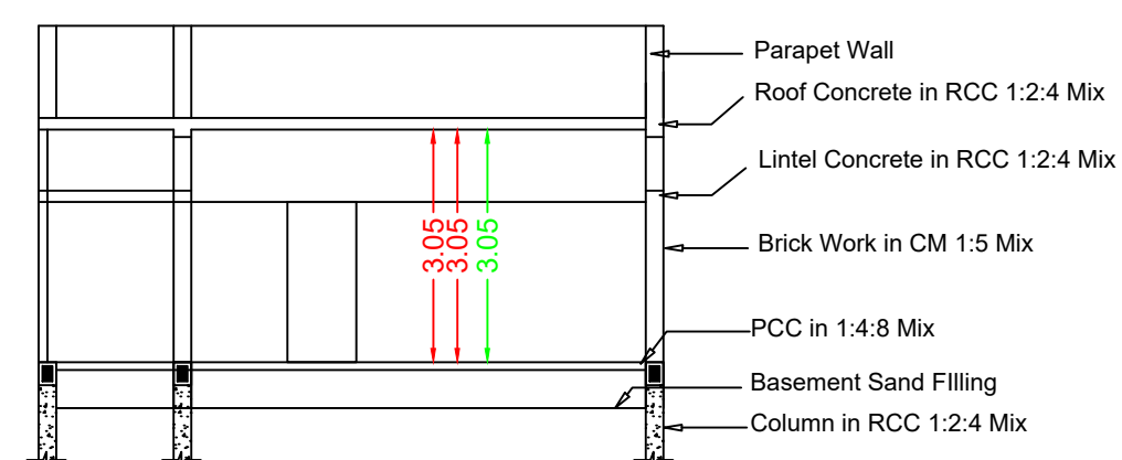
Section RR
