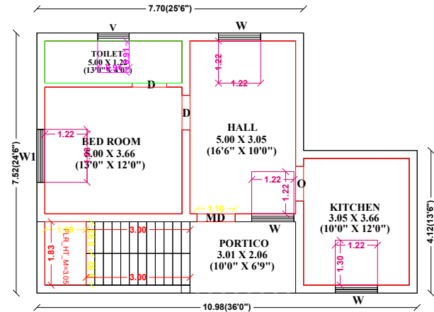
FLOOR-GROUND
