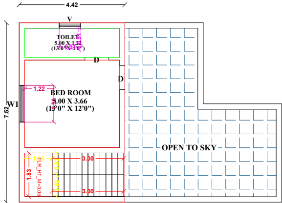
FLOOR-FIRST
