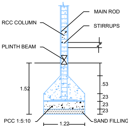
COLUMN DETAILS
