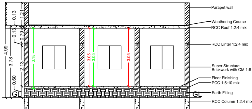
SECTION ON "VR"
