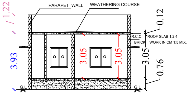
Section on-"AA"
