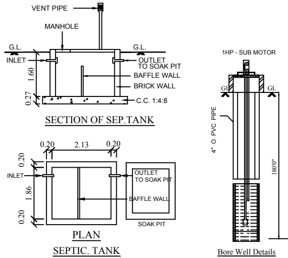
Bore Well Details
