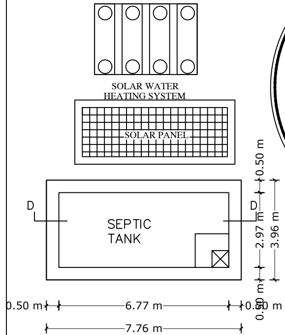
PLAN OF SEPTIC TANK SCALE 1"=2'0"
