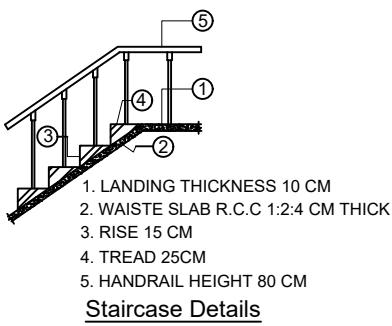
Staircase Details
