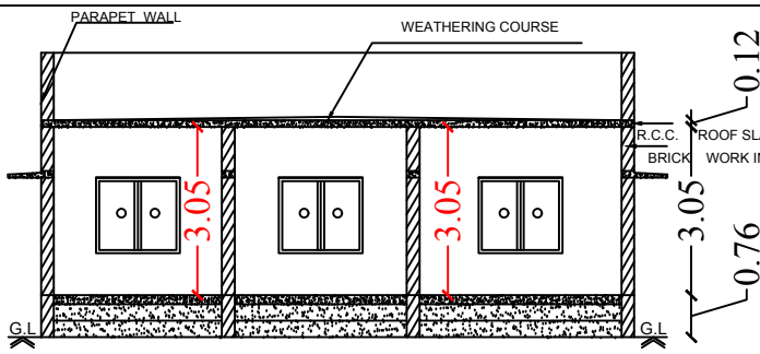
Section on-"AA"
