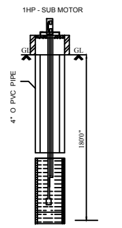
Bore Well Details
