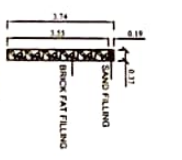
DETAILS OF PERCOLATION PIT
