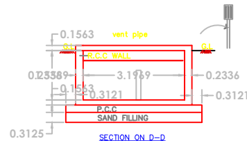
SECTION ON D-D
