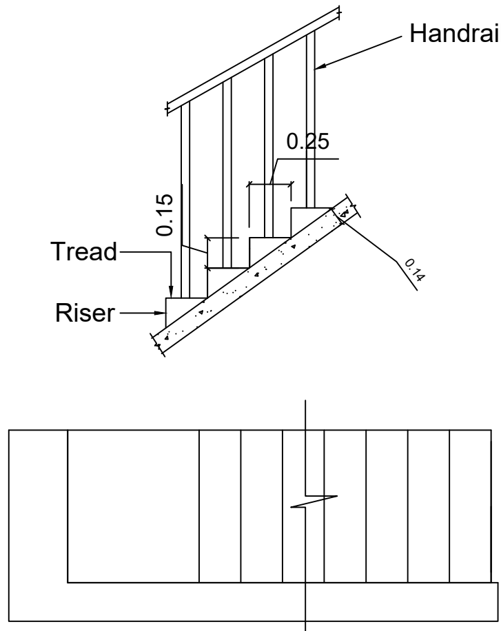
STAIRCASE DETAIL
