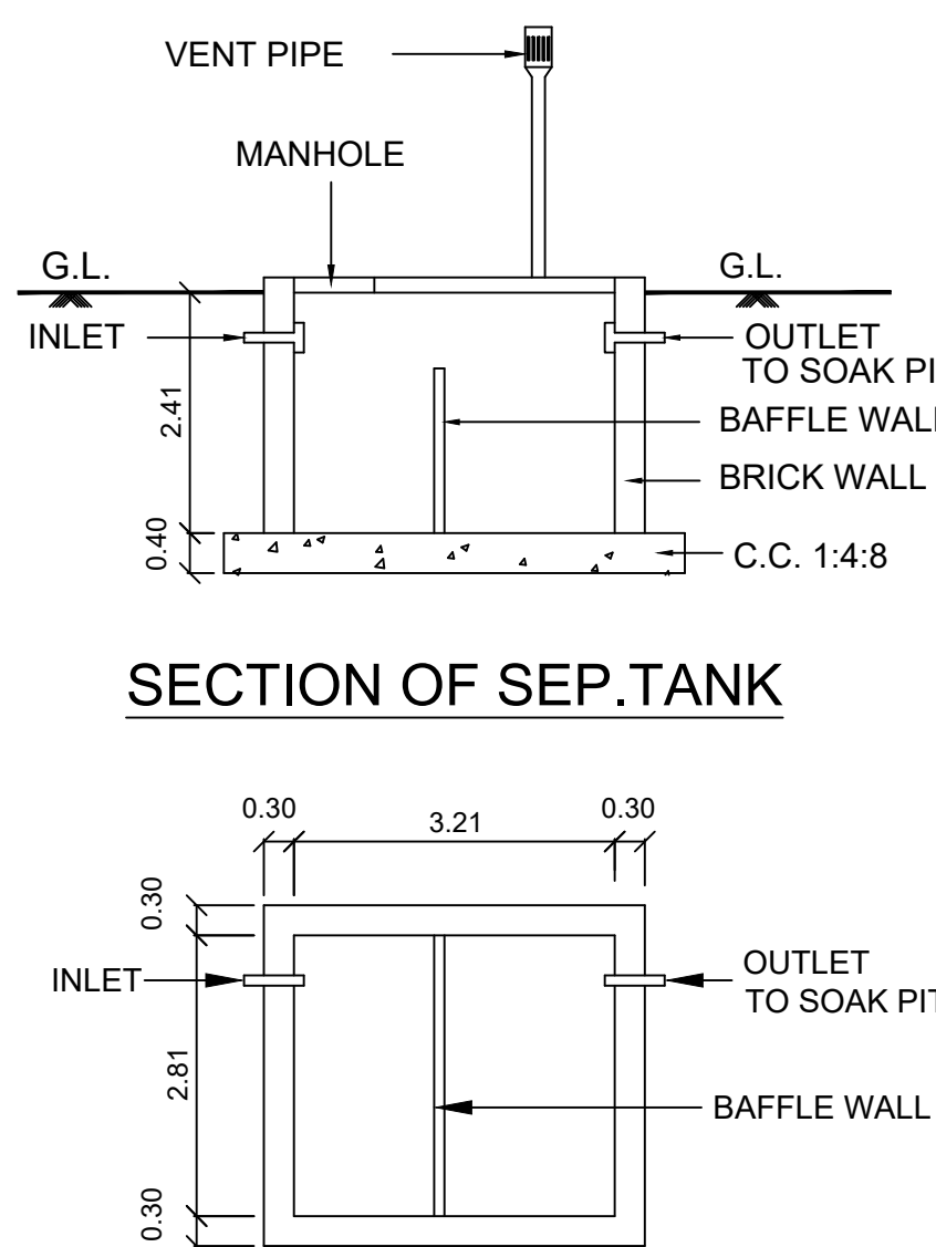
SEPTIC. TANK
