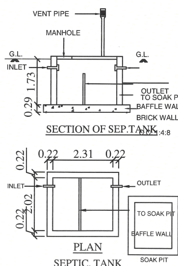
PLAN SEPTIC. TANK
