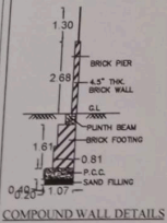
COMPOUND WALL DETAILS
