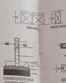
FOUNDATION DETAILS (Concentric Footing)
