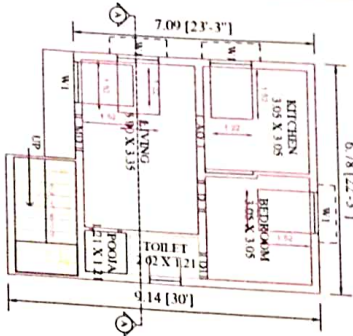
PROPOSED GROUND FLOOR PLAN
