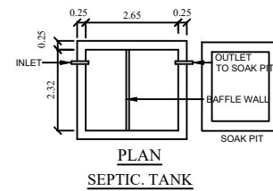
SEPTIC. TANK
