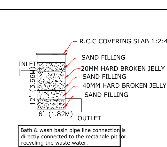
Waste Water Recycle Unit Not To Scale
