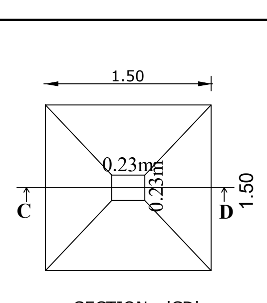
Isolated Footing -A (1.50X1.50) (Not to Scale)
