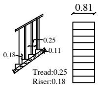
STAIRCASE DETAIL
