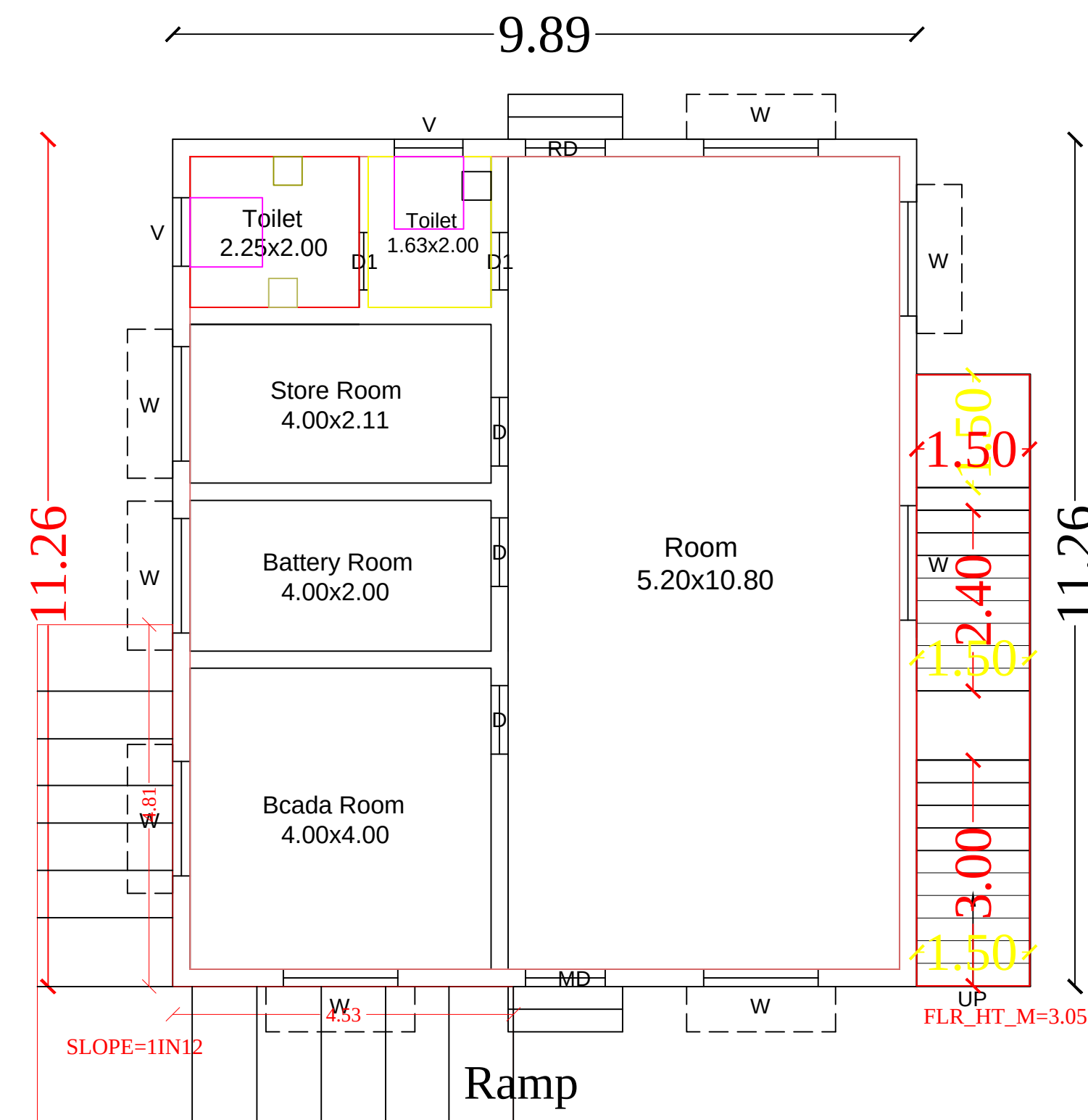
11.40 Ground Floor
