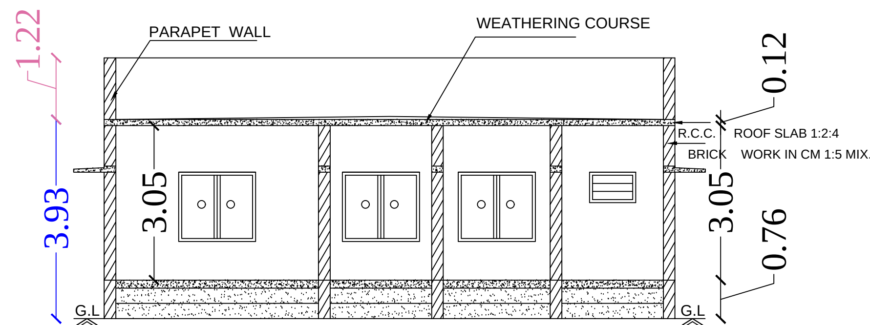
Section on-"AA"
