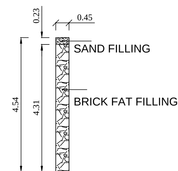
DETAILS OF PERCULATION PIT
