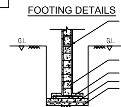
FOOTING DETAILS SECTION
