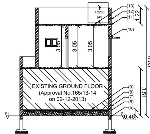
FIRST FLOOR SECTION "AA"
