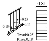
STAIRCASE DETAIL
