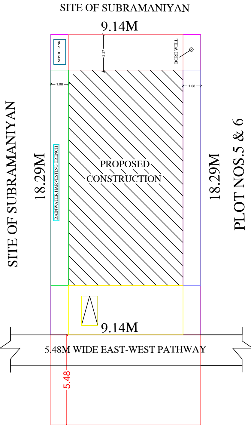
SITE PLAN
