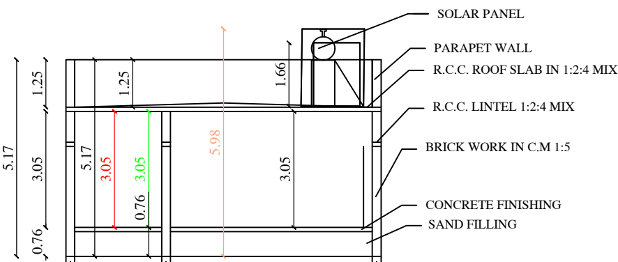
CUT SECTION ON AA
