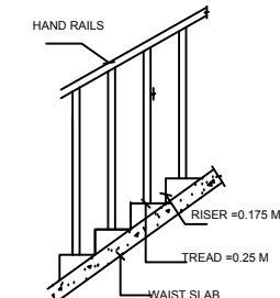
STAIR CASE DETAILS
