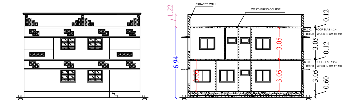
Front Elevation
