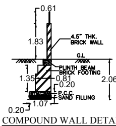
COMPOUND WALL DETAILS
