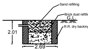
DETAILS OF RAIN WATER HARVESTING
