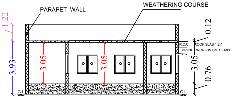
Section on-"AA"
