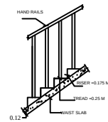
STAIR CASE DETAILS
