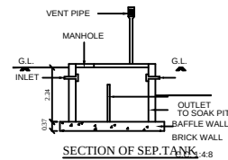
SECTION OF SEP. TANK
