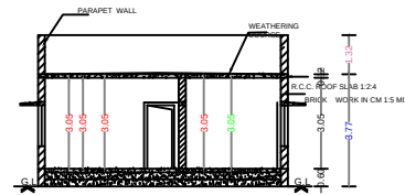
Section on-"AA"
