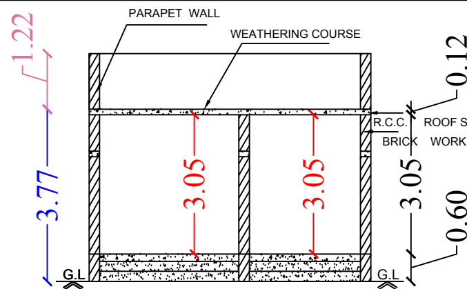
Section on-"AA"
