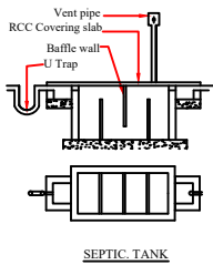
SEPTIC TANK
