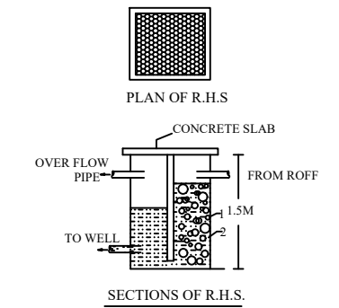
SECTIONS OF R.H.S.
