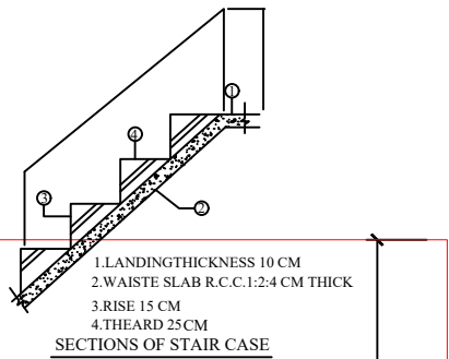
SECTIONS OF STAIR CASE
