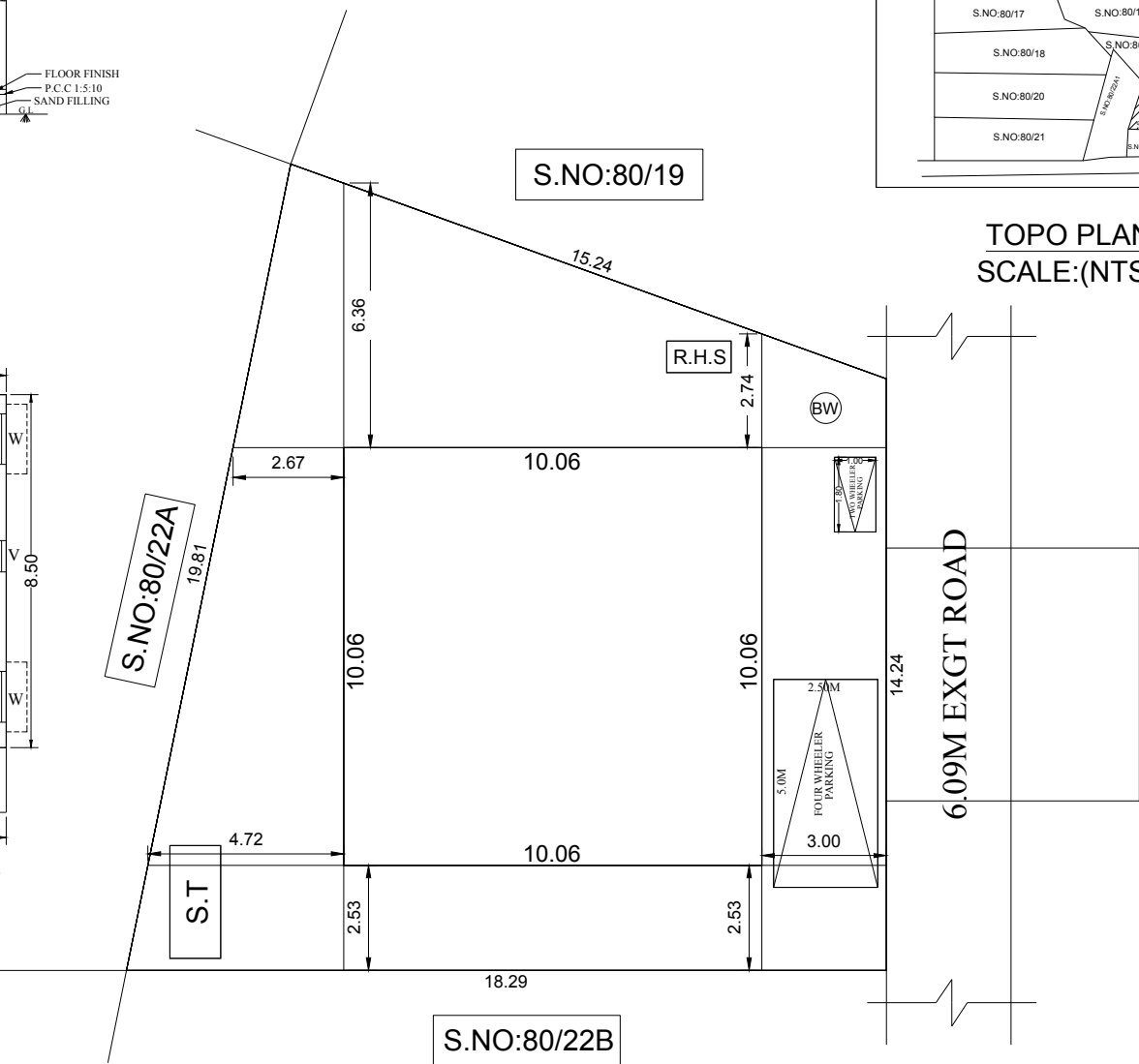
SITE PLAN
