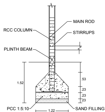
COLUMN DETAILS
