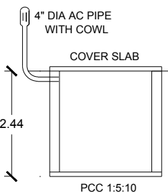
SEPTIC TANK
