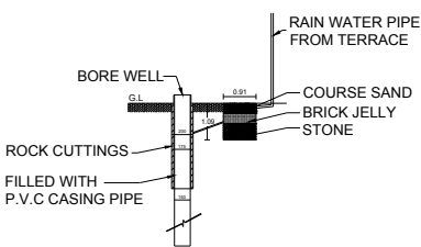
RAIN WATER HARVESTING DETAIL
